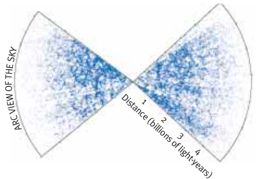
TWO-DEGREE FIELD GALAXY REDSHIFT SURVEY AND ANGLO-AUSTRALIAN OBSERVATORY
