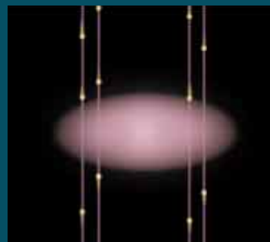
The generation of jets may begin when material—a mixture of ions, atoms, molecules and dust—rains onto the circumstellar disk along magnetic field lines.
