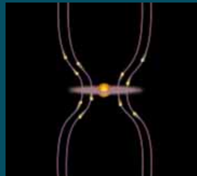
When the field lines are bent to an angle of 30 degrees from the perpendicular, centrifugal force overcomes gravity and flings material outward along the lines.
