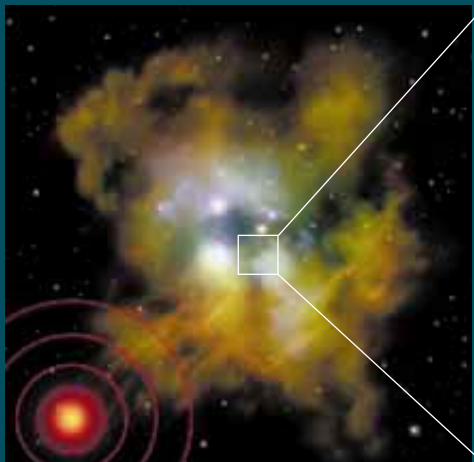
A star begins to coalesce when a disturbance, such as a nearby supernova explosion, causes a cloud of gas and dust to collapse.
